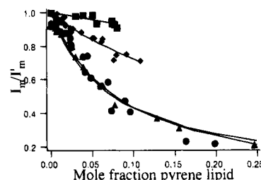
FIGURE 3: Dependence of the normalized monomeric fluorescence intensity on the mole fraction of incorporated pyrene-labeled PC (●), PI (▲), PIP (◆), and PIP 2 (■) in DOPC vesicles. The curves are the best fits obtained by applying eqs 2 and 6 to the experimental points, giving results listed in Table 2. The experiments were performed at 20 °C.
